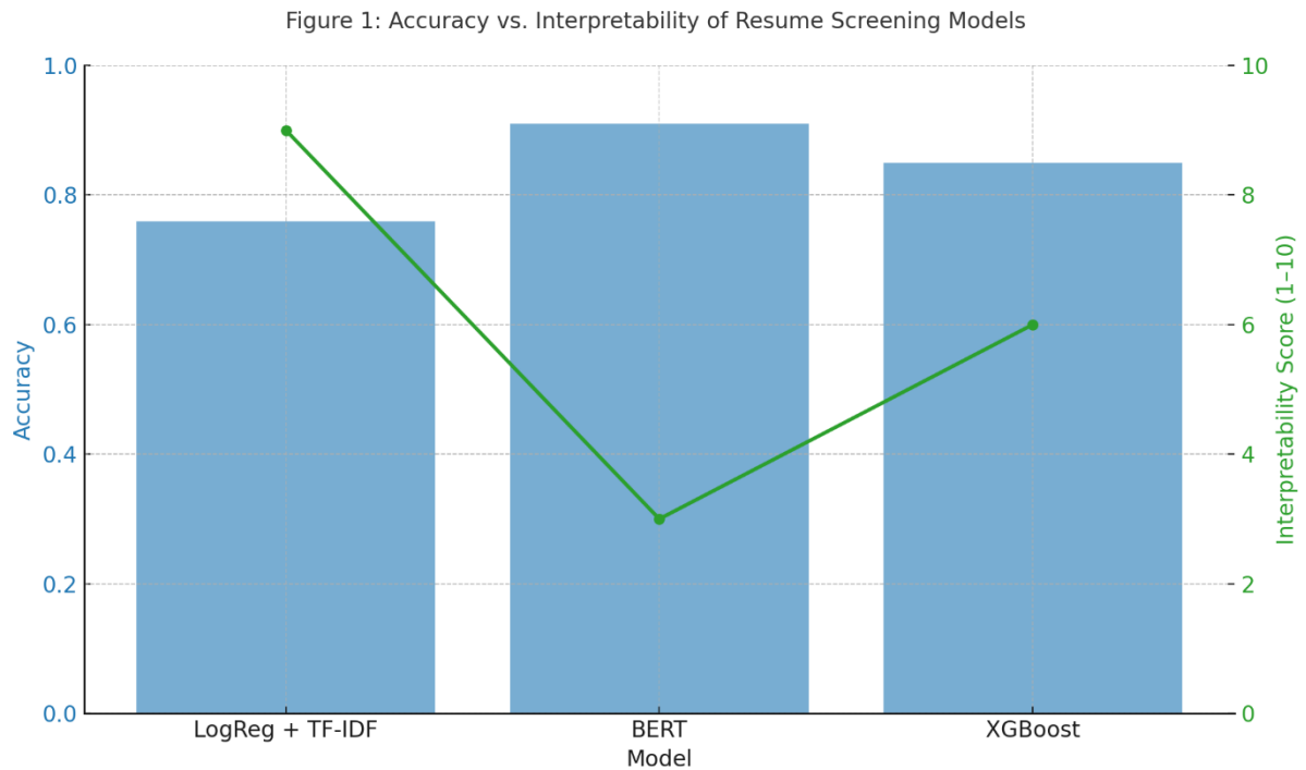
Figure 1. Comparison of classification accuracy and interpretability across three resume screening models. While BERT achieves the highest accuracy (91%), it ranks lowest on interpretability. Logistic Regression with TF-IDF, though less accurate, offers the highest transparency, making it preferable for auditability and compliance-sensitive deployments.
