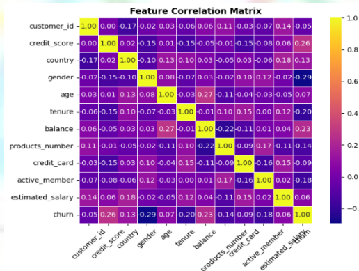
Figure 3: Correlation feature heatmap of Bank Customers Churn Dataset
