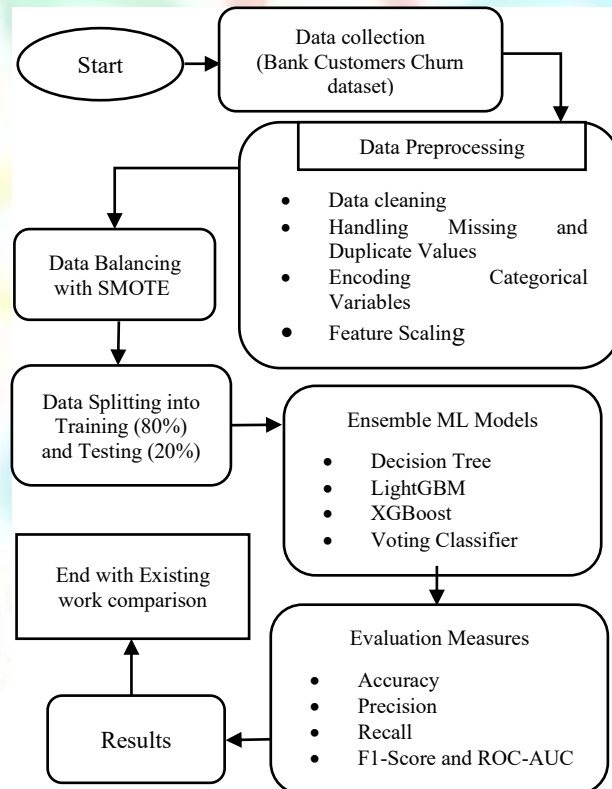
Figure 1: Proposed Flowchart for customer churn prediction using ML models
