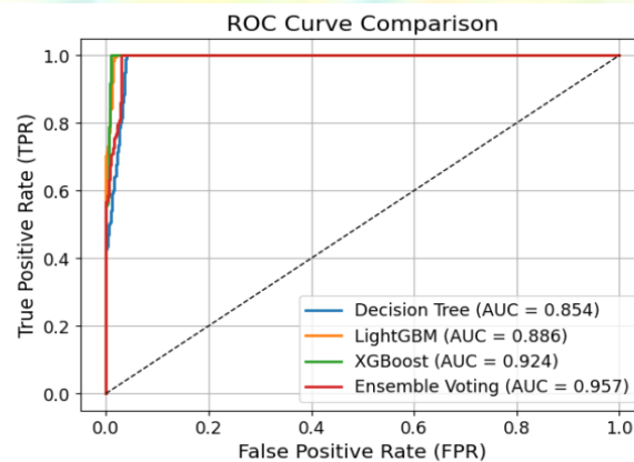
Figure 6: ROC Curve of Proposed Models for Churn Prediction
