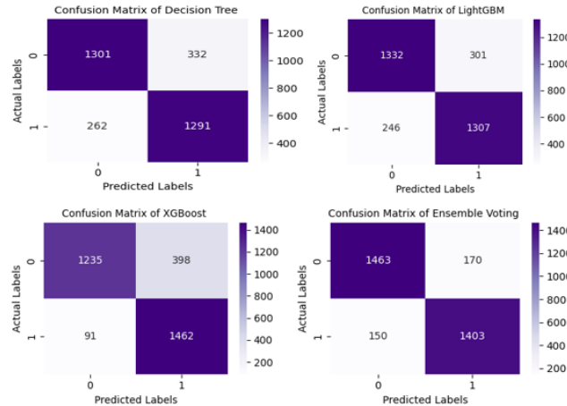
Figure 5: Confusion Matrix of Proposed Models for Churn Prediction
